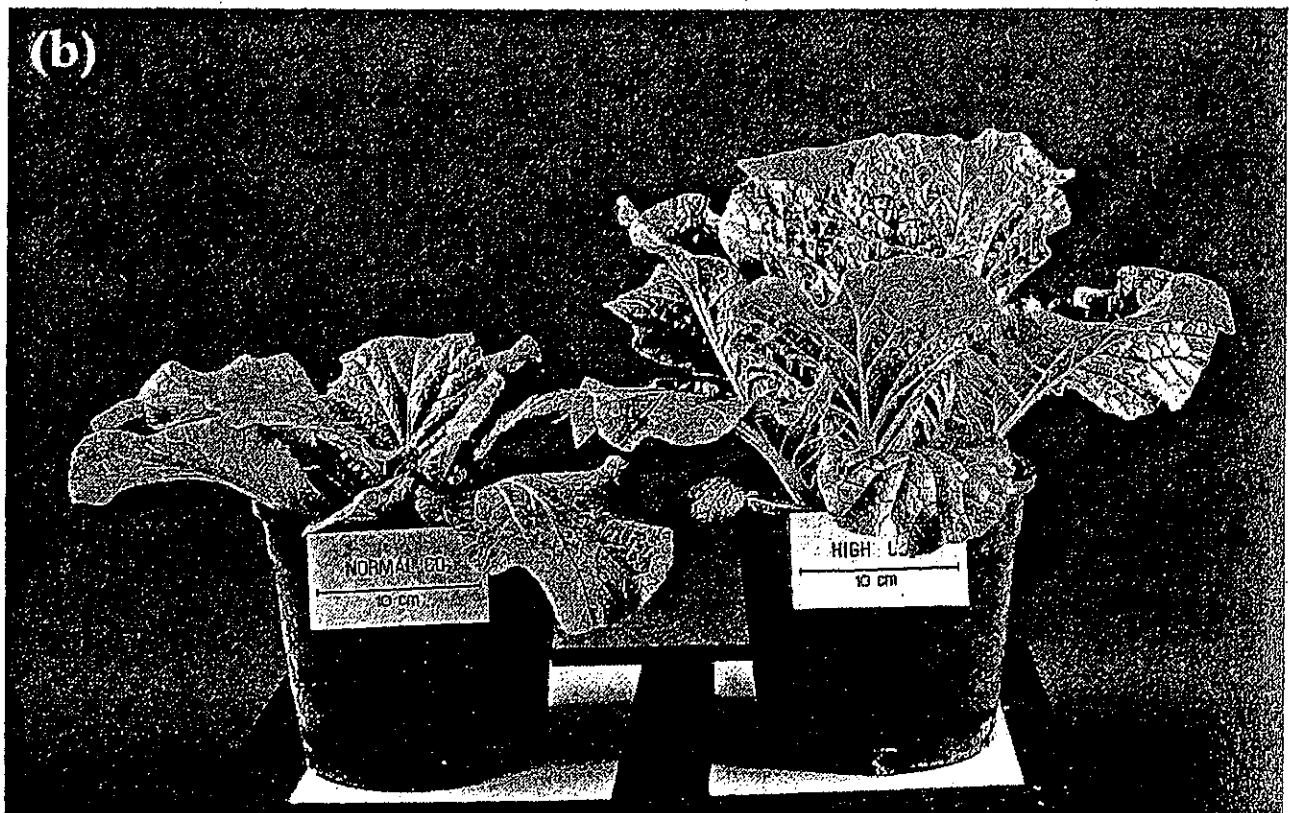
Figure 6:10 Early growth of cucumber ( Cucumis sativus ) (a) and wong bok ( Brassica pekinensis ) (b) is greatly enhanced in elevated \text{CO}_2 (1250 ppm) compared with ambient controls (325 ppm). As shown here, that initial effect is still apparent after 52 d of greenhouse culture in nutrient-rich potting mix. Scale bar = 10 cm. (Further details in Kriedemann and Wong (1984) and Table 6.4)
